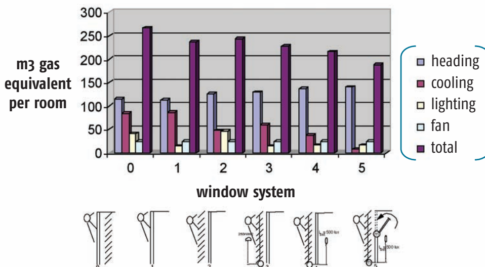
Figure 5. Primary energy per room needed for heating, cooling, lighting and transport.
