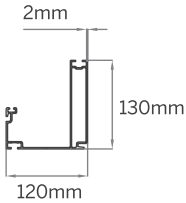
② Gutter
