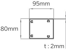
③ Post
